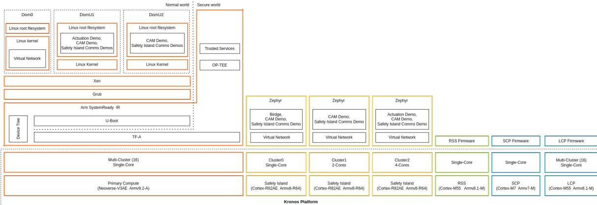
Arm Kronos Reference Software Stack High-Level Diagram - Virtualization Architecture
