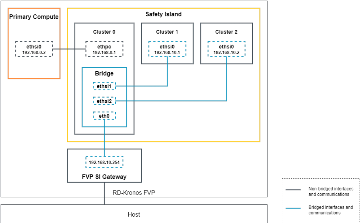
Safety Island Cluster 0 Bridge High-Level Diagram
