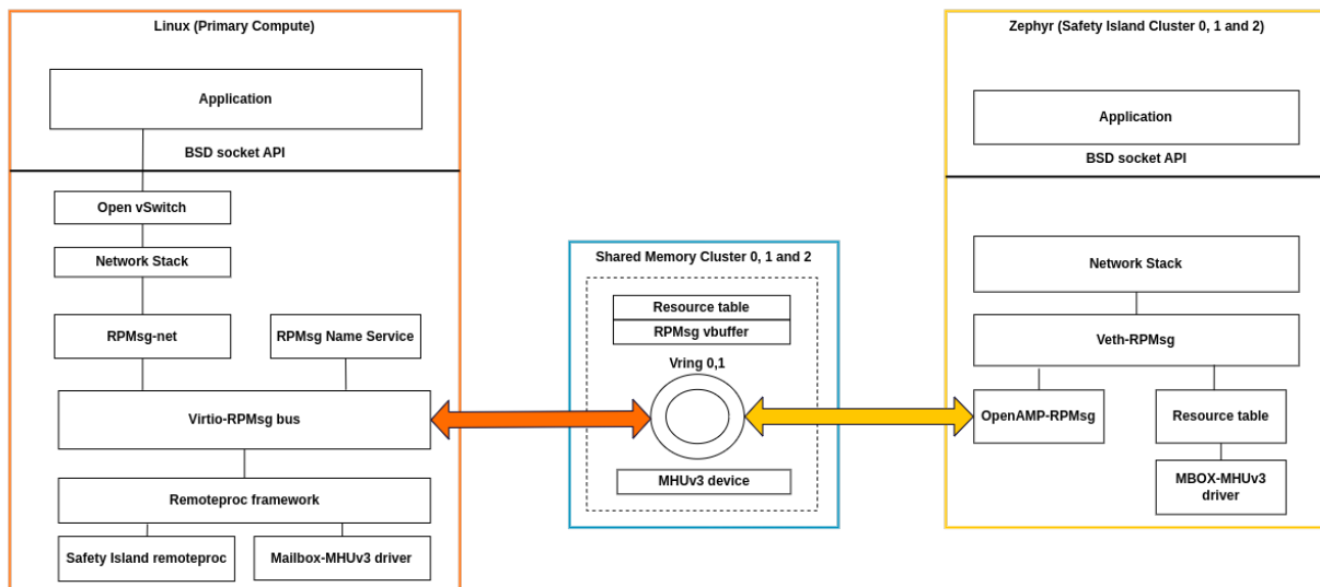
Arm Kronos Reference Software Stack HIPC - Baremetal Architecture
