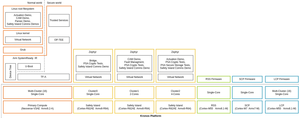
Arm Kronos Reference Software Stack High-Level Diagram - Baremetal Architecture
