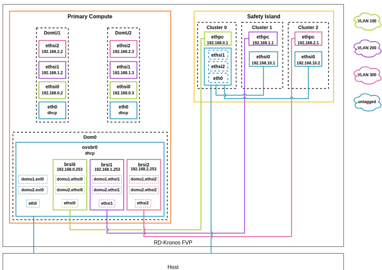
Arm Kronos Reference Software Stack Network Topology - Virtualization Architecture
